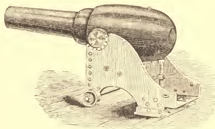
Fig. 10.—Whitworth Gun.
